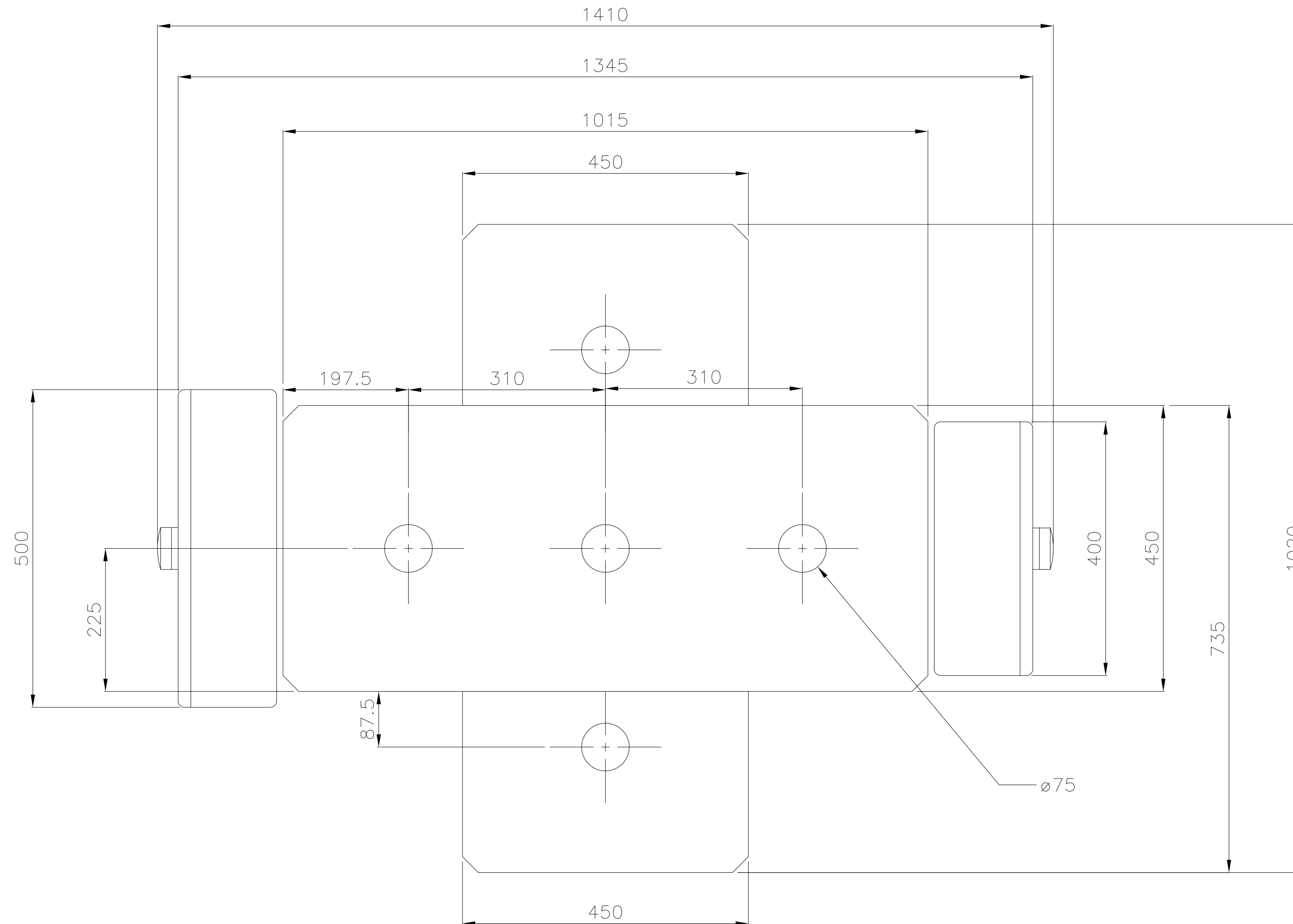
PLAN
